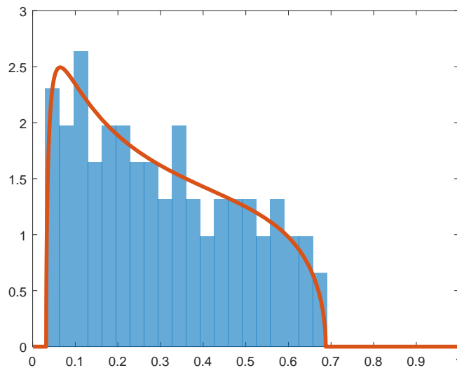
Figure 7: Eigenvalues from S&P data and Wachter distribution.
