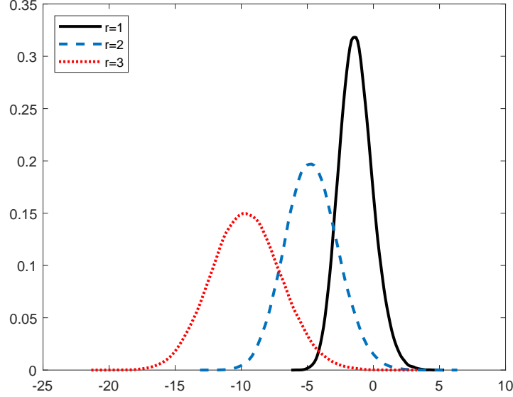
Figure 1: The probability density for the random variables \sum_{i=1}^r \alpha_i . The histogram plots are obtained from 100,000 samples of 200 \times 200 Gaussian matrices following Proposition 1.
